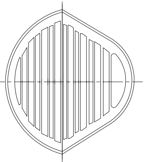
UNDERSIDE
